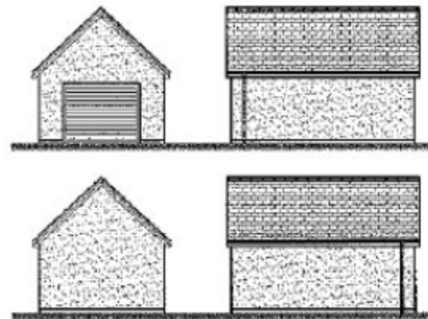
Garage elevations 1:250
